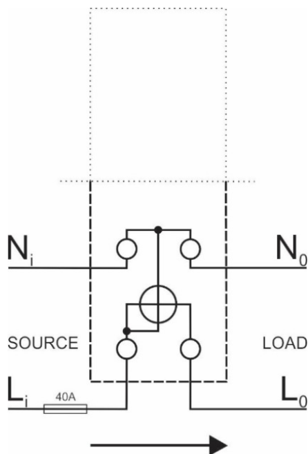
Figure 1: Connection diagram
