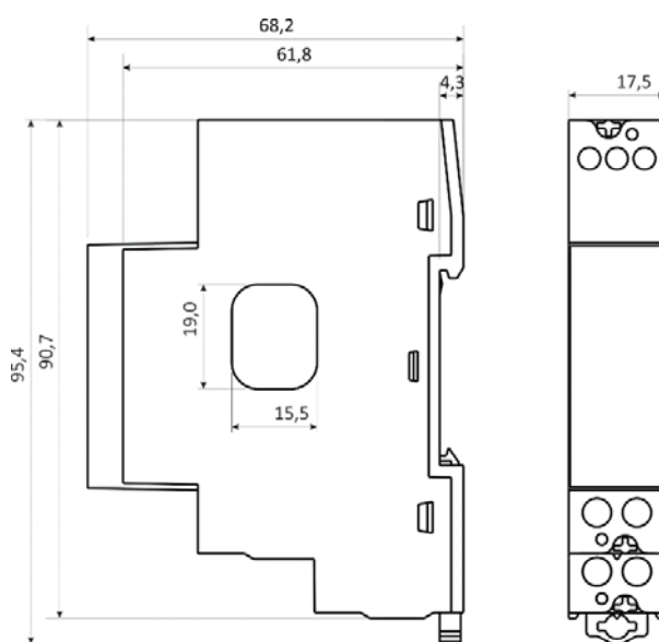
Figure 3: Dimensional drawing of IE14xx
